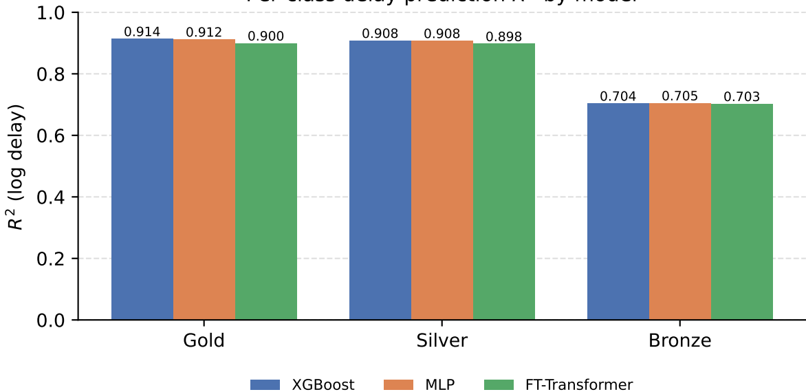
Per-class delay prediction R^2 by model
